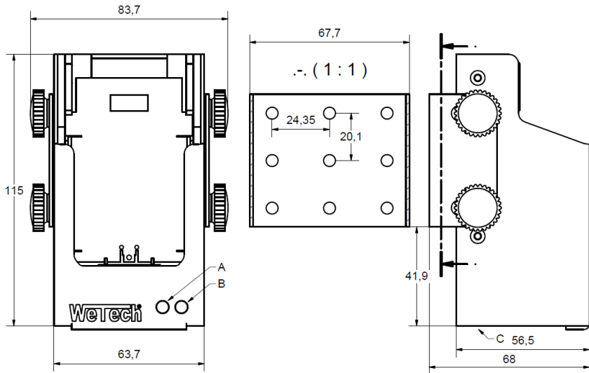
Schematic drawing WTC1702
